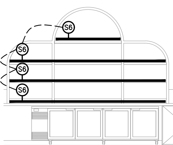
DETAIL GR2 GAMING BAR REAR WALL SCALE 1: 50
